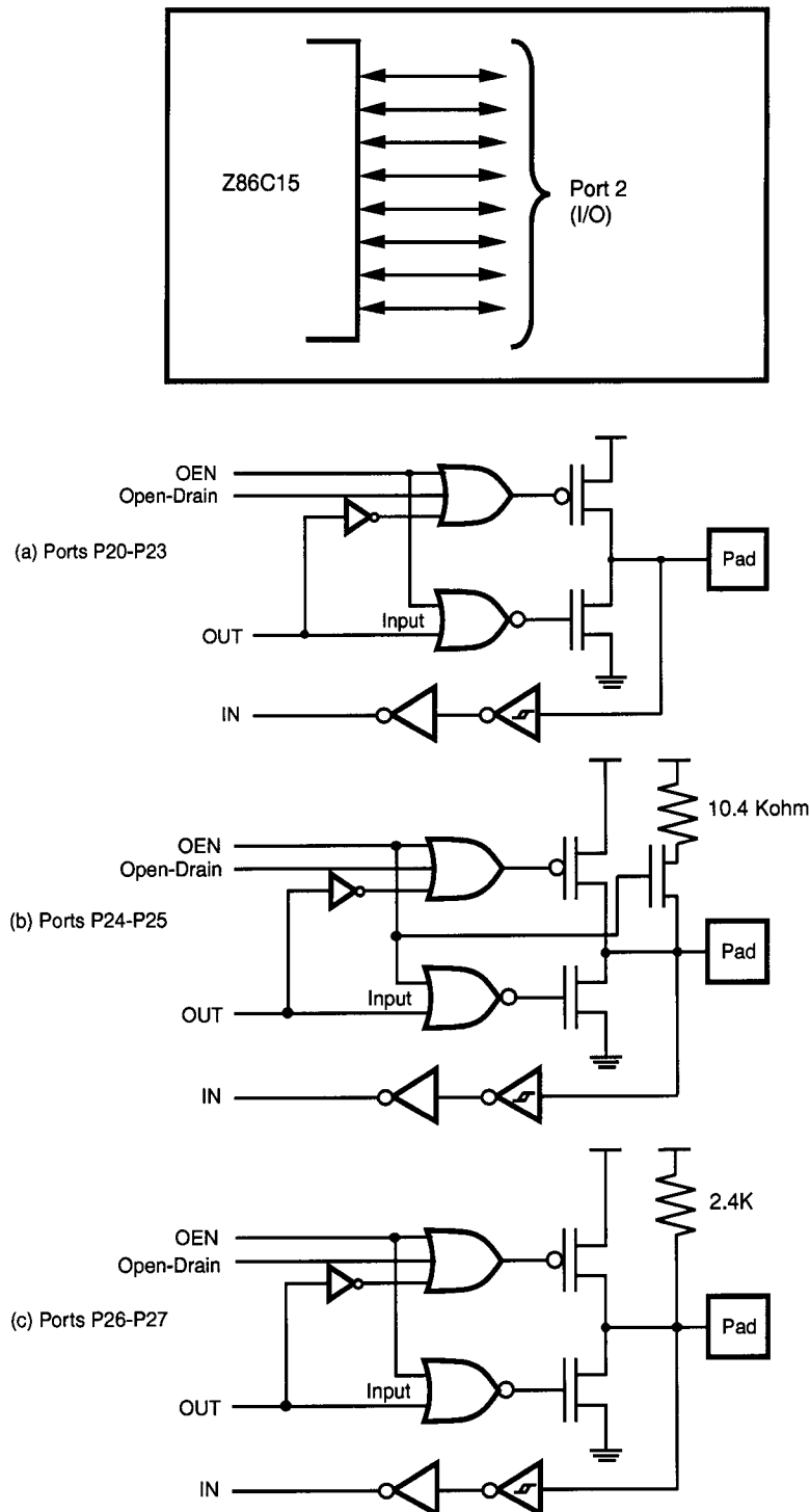
Figure 9. Port 2 Configuration
