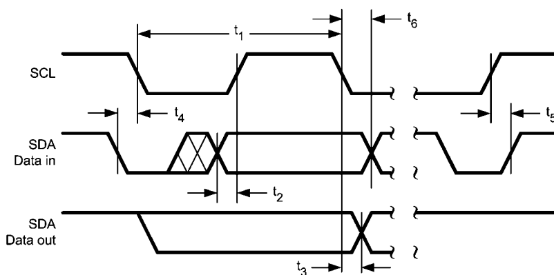
FIGURE 3. I 2 C Timing Diagram
