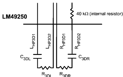
FIGURE 7. External 3D Effect Capacitors
