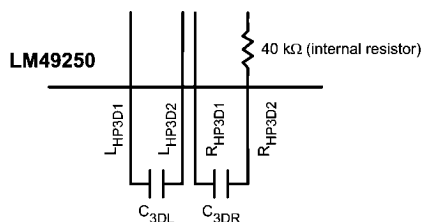
FIGURE 6. External RC Network with Optional R_{3DL} and R_{3DR}
