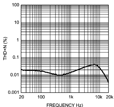
THD+N vs Frequency Single-ended Input, Headphone Mode 2 V_{DD} = 3.6V , P_{OUT} = 30mW , R_L = 16\Omega
