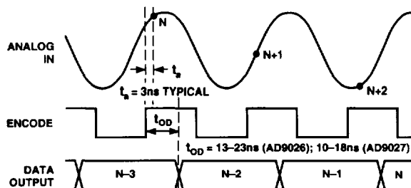
Figure 20. Timing Diagram
