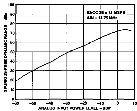
Figure 10. SFDR vs. Analog Input Level
