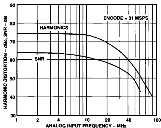
Figure 13. Noise and Distortion vs. AIN Frequency
