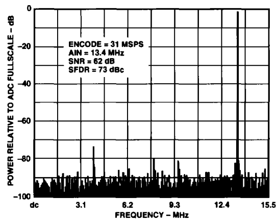
Figure 7. Single Tone at 13.4 MHz
