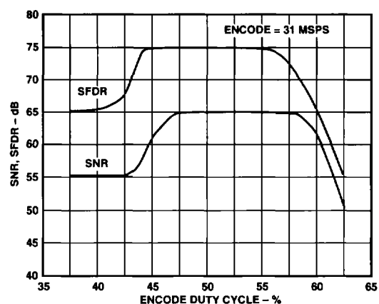
Figure 17. SNR, SFDR vs. Encode Duty Cycle
