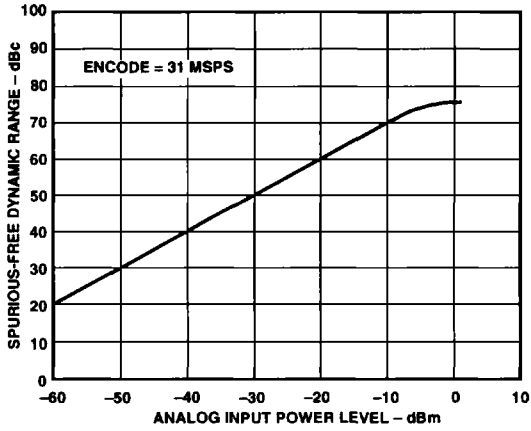
Figure 11. Two-Tone SFDR vs. Analog Input Level
