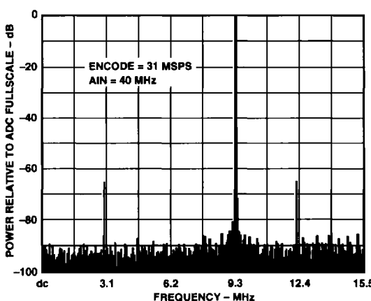
Figure 12. Undersampling a 40 MHz Input Tone
