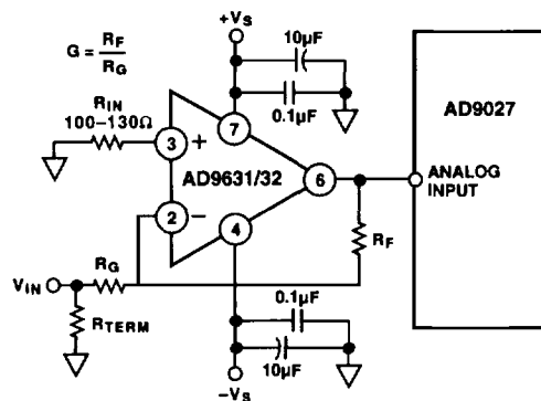
Figure 21. Low Distortion Drive Circuit for AD9026/AD9027
