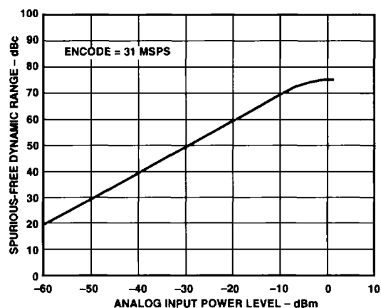
Figure 5. Two-Tone SFDR vs. Analog Input Level
