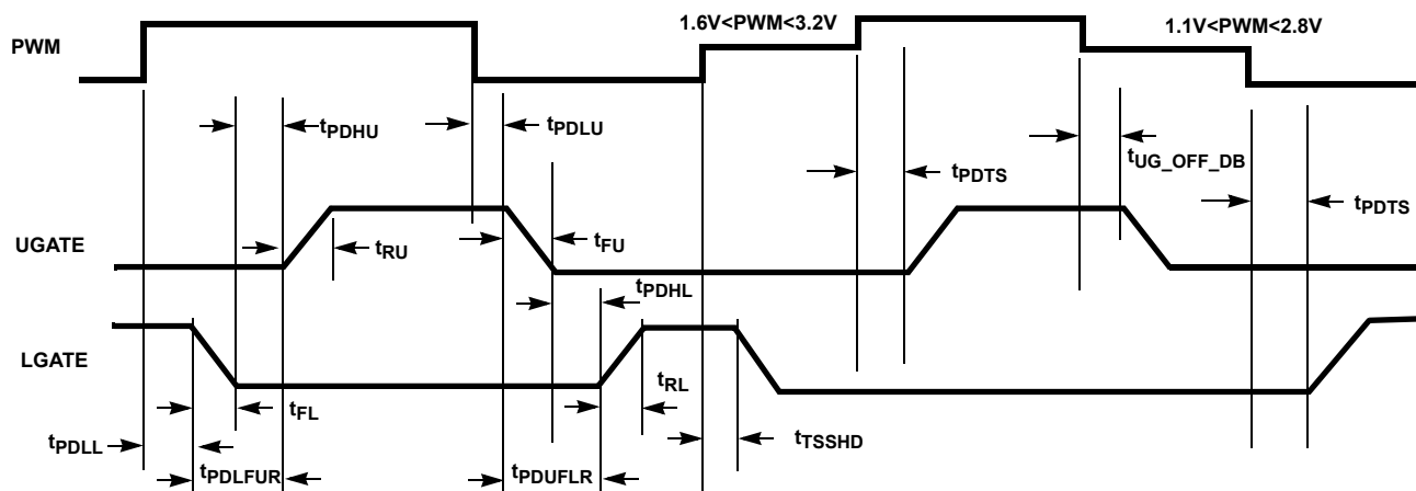
FIGURE 2. TIMING DIAGRAM
