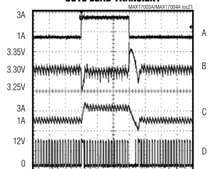
OUT3 LOAD TRANSIENT
