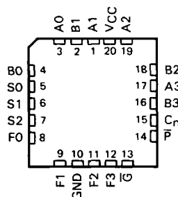
SN54F381 . . . FK PACKAGE (TOP VIEW)
