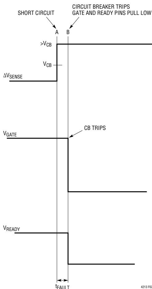
Figure 2. Short Circuit Fault Timing Diagram
