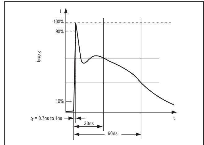
Figure 7b. IEC 1000-4-2 ESD Generator Current Waveform
