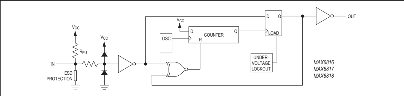
Figure 1. Block Diagram
