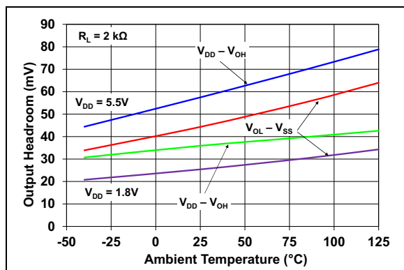
FIGURE 2-18: Output Voltage Headroom vs. Ambient Temperature.
