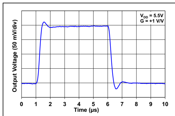
FIGURE 2-42: Noninverting Small Signal Step Response.
