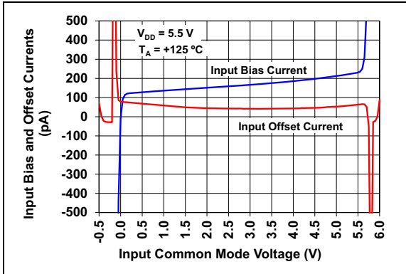
FIGURE 2-13: Input Bias and Offset Currents vs. Common Mode Input Voltage with T_A = +125\text{ }^{\circ}\text{C} .
