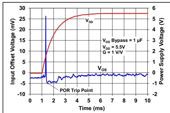
FIGURE 2-40: Input Offset Voltage vs. Time at Power-Up.
