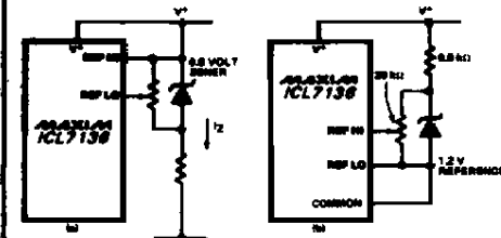
Figure 4. Using an External Reference
