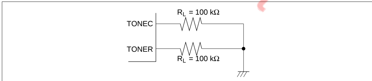
Figure 48 Tone Output Load Circuit
