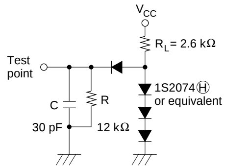
Figure 54 Timing Load Circuit
