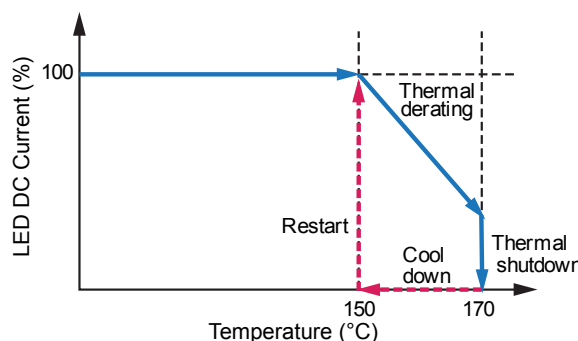
Figure 9: Thermal Derating and Shutdown Protection Features
