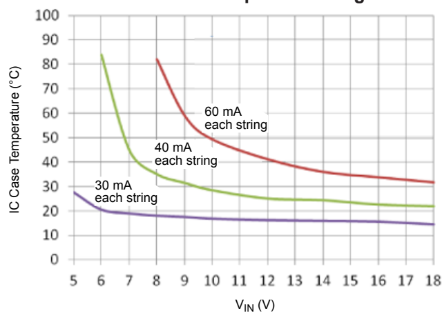
Temperature Rise versus V_{IN} 8 series LEDs in 8 parallel strings
