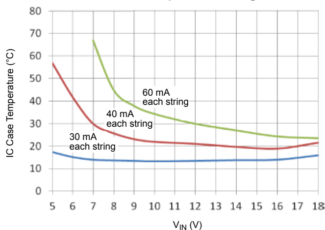
Temperature Rise versus V_{IN} 7 series LEDs in 8 parallel strings
