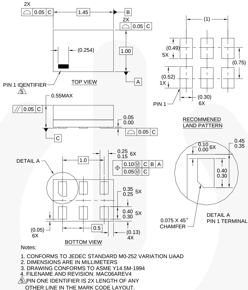
Figure 16. 6-Lead, Micropak™ 1.0 mm Wide Package
