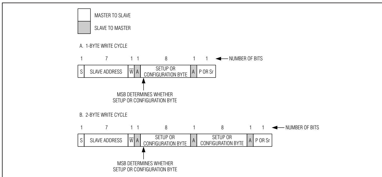
Figure 9. Write Cycle
