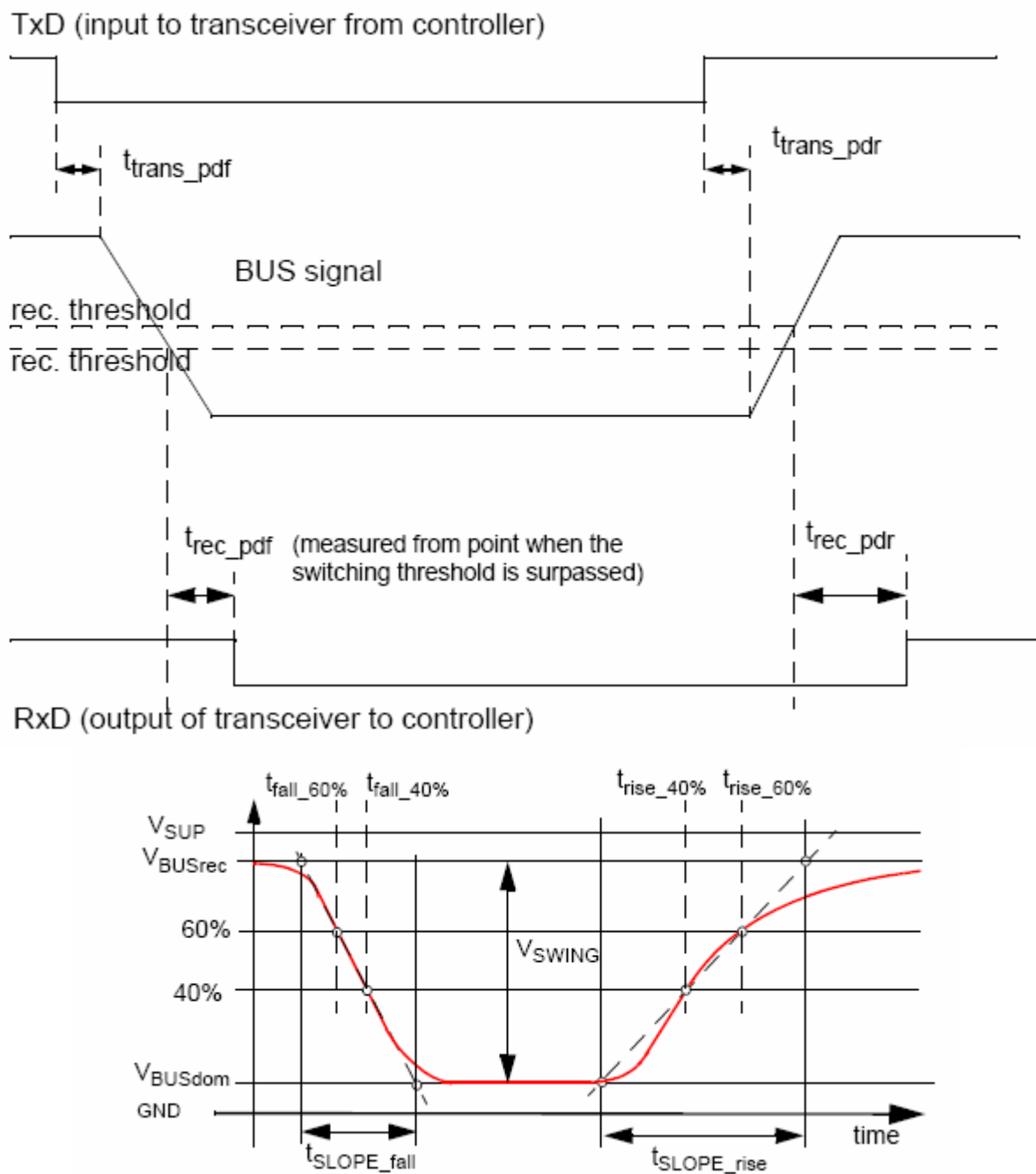
Figure 6 : LIN V1.3 Timing Specification
