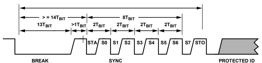
Figure 39: LIN Interface Timing
