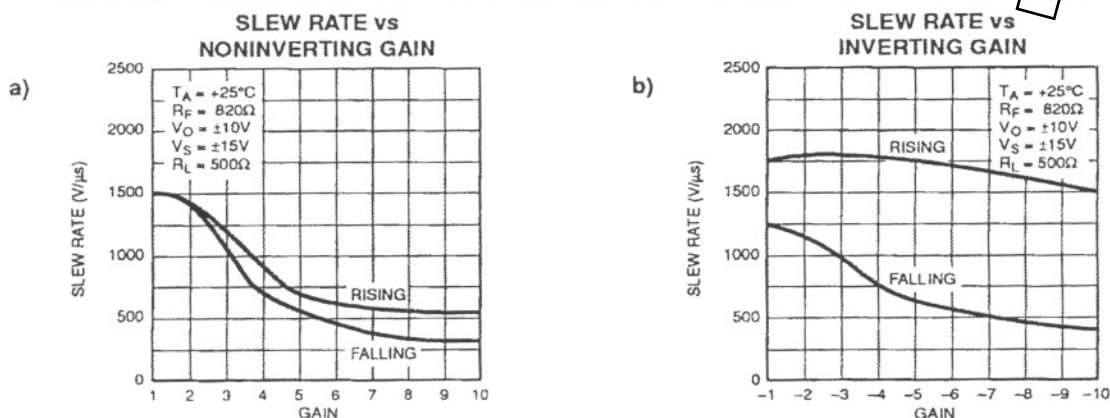
FIGURE 6: Slew rate of the OP-160 in noninverting (a) and inverting (b) configurations.
