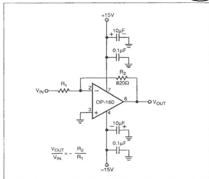
FIGURE 21: The OP-160 as an inverting amplifier.
