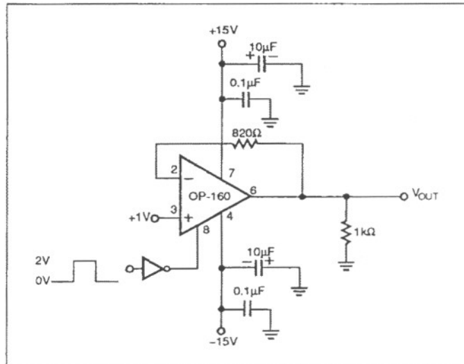
FIGURE 16: DISABLE Turn-On/Turn-Off Test Circuit
