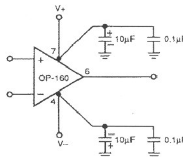
FIGURE 9: Proper power supply bypassing is required to obtain optimum performance with the OP-160.
