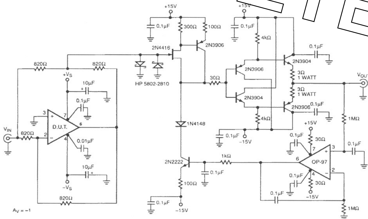
FIGURE 10: High-Speed Settling Time Fixture (for 0.1 and 0.01%)
