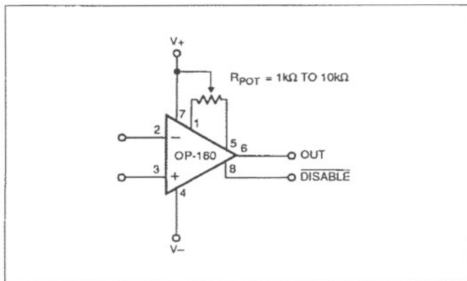
FIGURE 14: Input Offset Voltage Nulling
