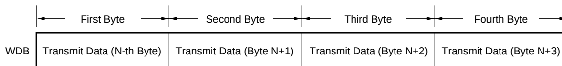
Figure 7-2. Data Exchange During Master Transmission (Contents of Write Data Buffer)
