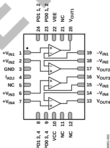
Figure 2. AD8394ACPZ, 24-Lead LFCSP, 4\text{ mm} \times 5\text{ mm}
