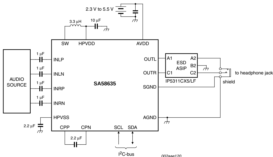
Fig 25. Typical application
