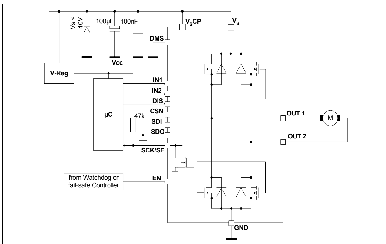
Figure 15 Application Example with Status-Flag
