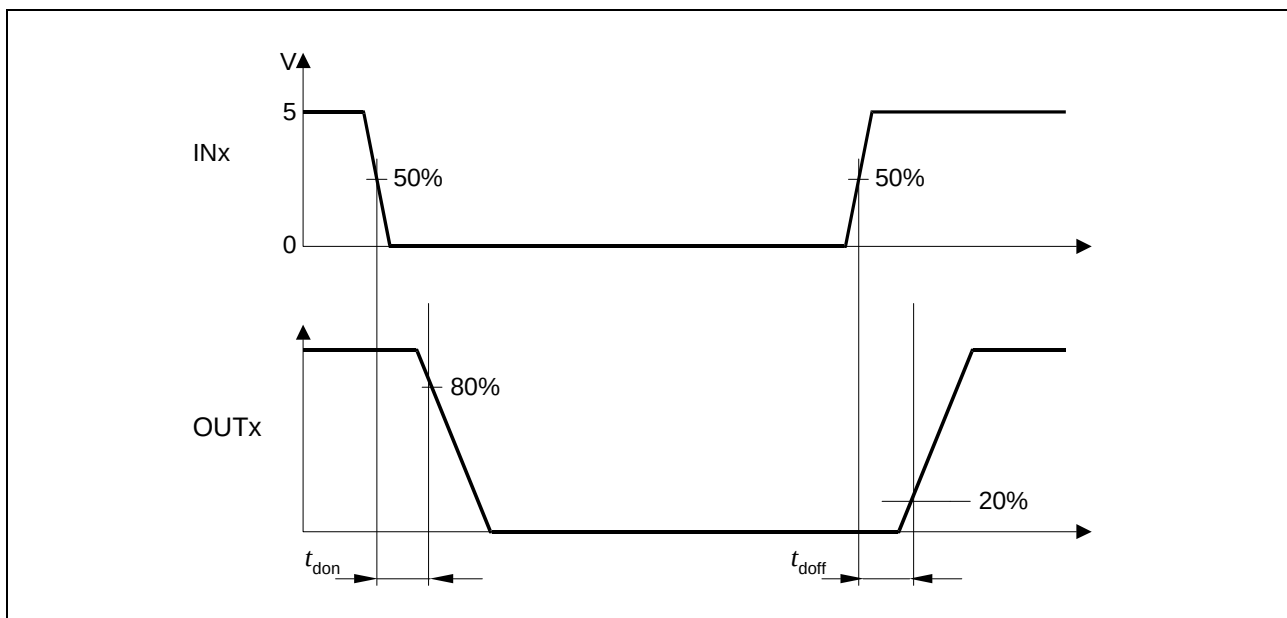
Figure 10 Output Delay Time--Depicted for Low-Side FETs
