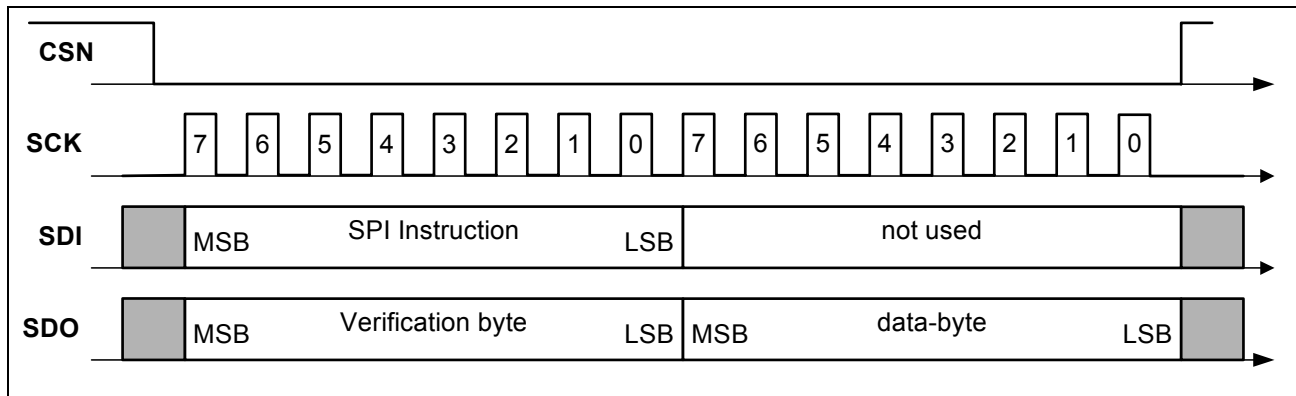
Figure 8 SPI communication
