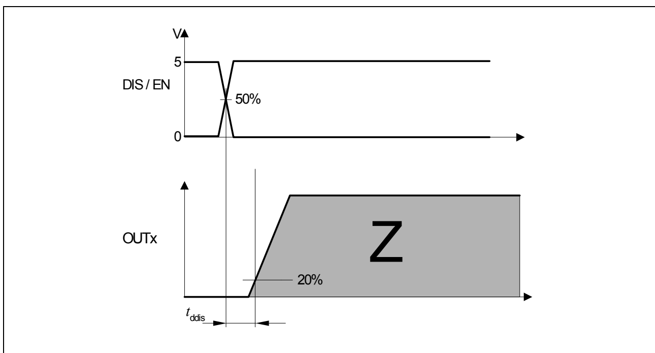
Figure 11 Disable Delay Time
