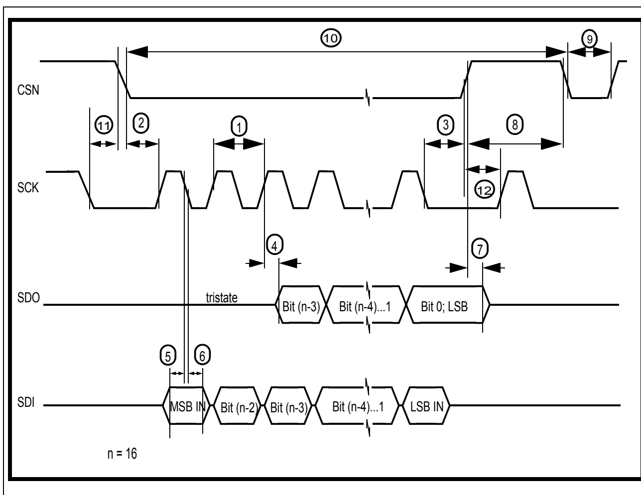
Figure 13 SPI-timing
