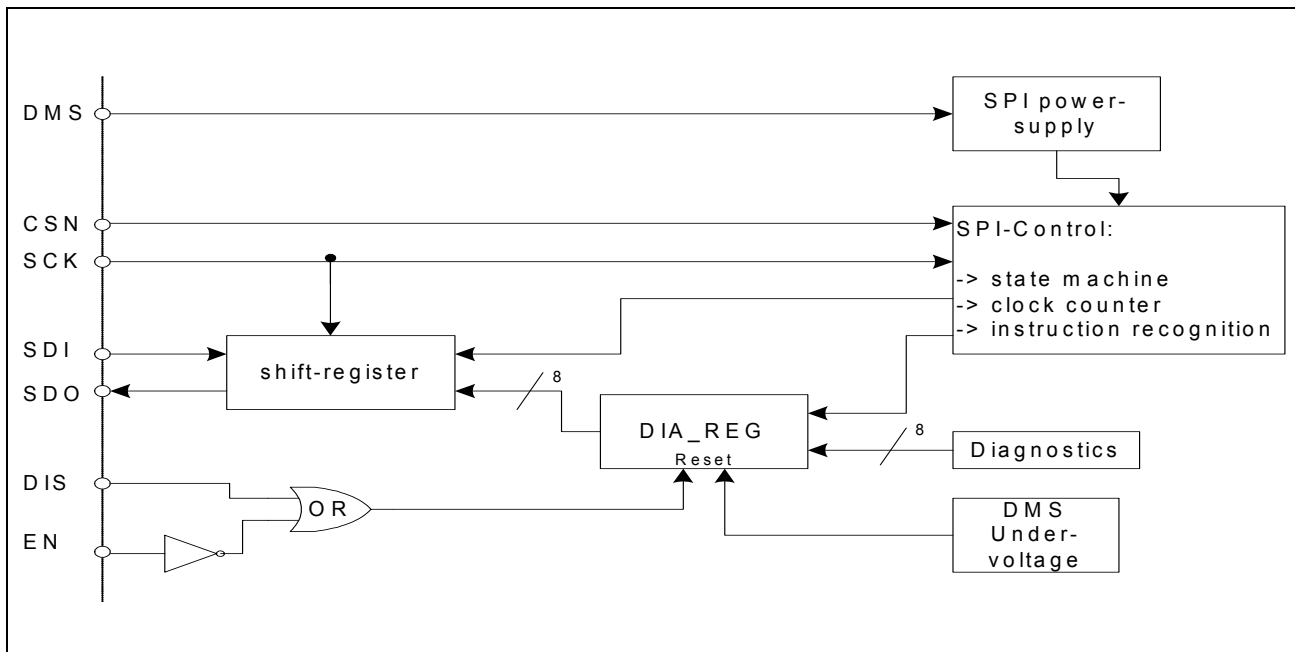
Figure 6 SPI block-diagram
