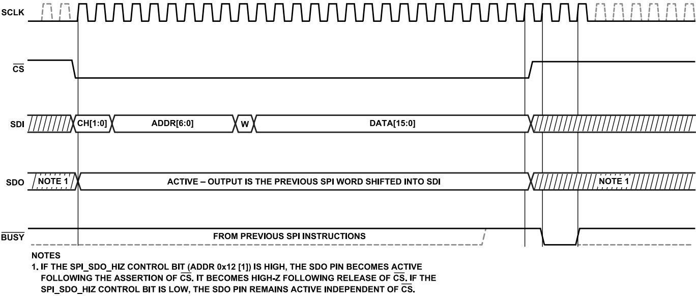
Figure 3. SPI Write Instruction Timing Diagram
