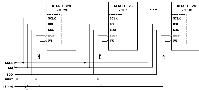
Figure 127. Multiple SPI with a Shared SDO Line
