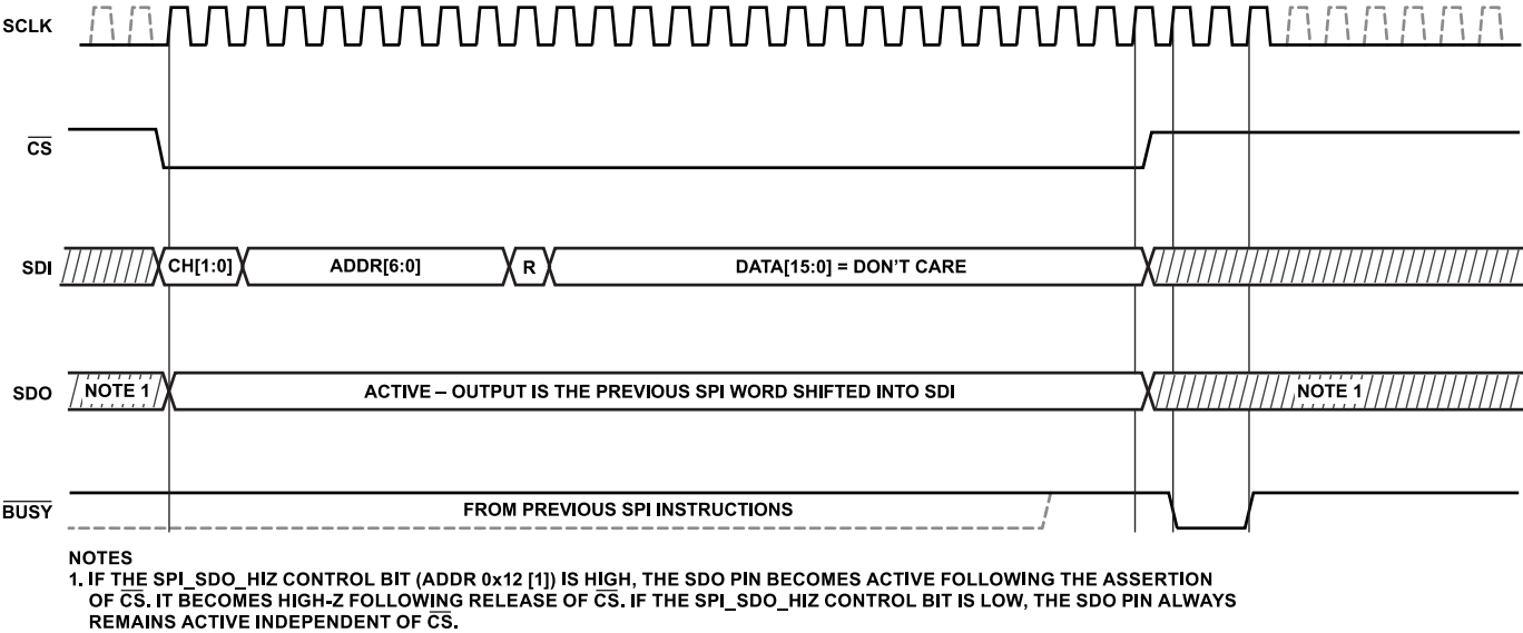
Figure 4. SPI Read Request Instruction Timing Diagram (Prior to Readout Instruction)
