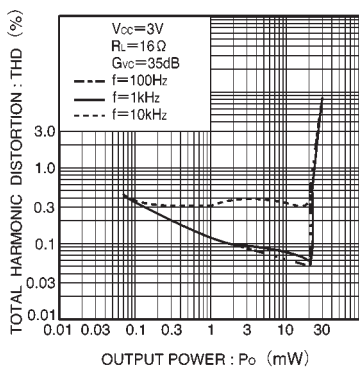
Fig. 5 Distortion vs. output power
