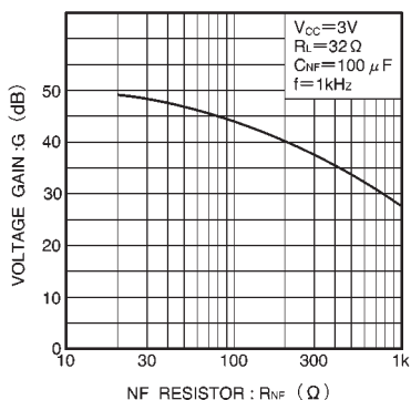
Fig. 13 Voltage gain vs. feedback resistor value
