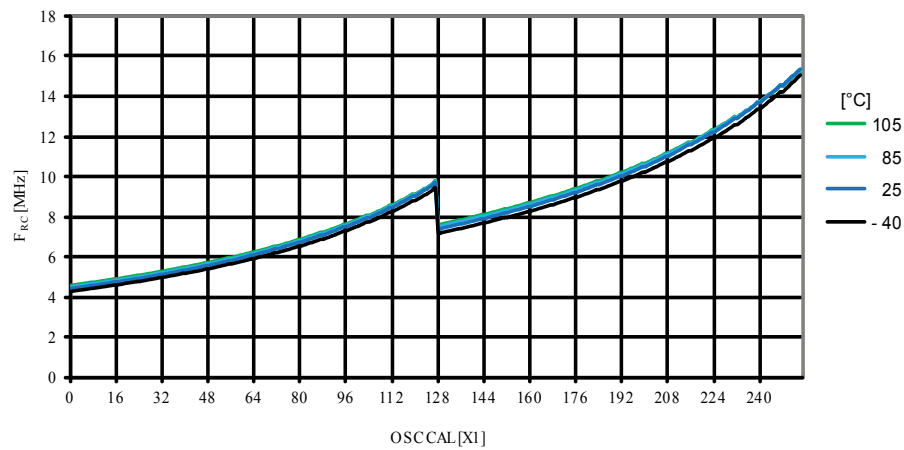
Figure 30-40. Calibrated 8MHz RC Oscillator vs. OSCAL Value
