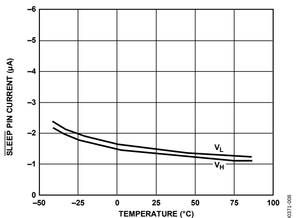
Figure 8. SLEEP Pin Current vs. Temperature
