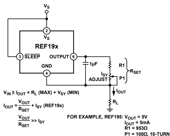
Figure 27. A Low Dropout, Precision Current Source
