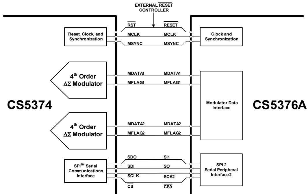
Figure 12. CS5374 to CS5376A Digital Interface
