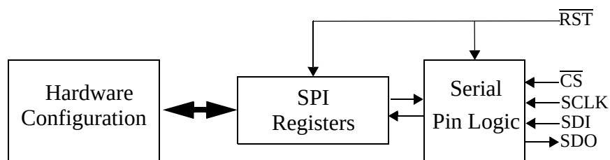
Figure 15. SPI Interface Block Diagram
