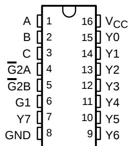
CD54ACT138 . . . F PACKAGE CD74ACT138 . . . E OR M PACKAGE (TOP VIEW)
