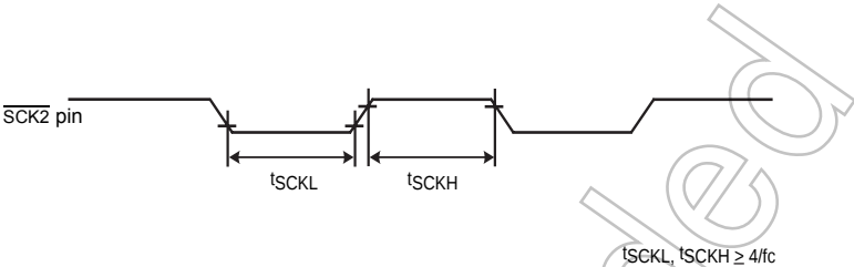
Figure 15-3 External Clock
