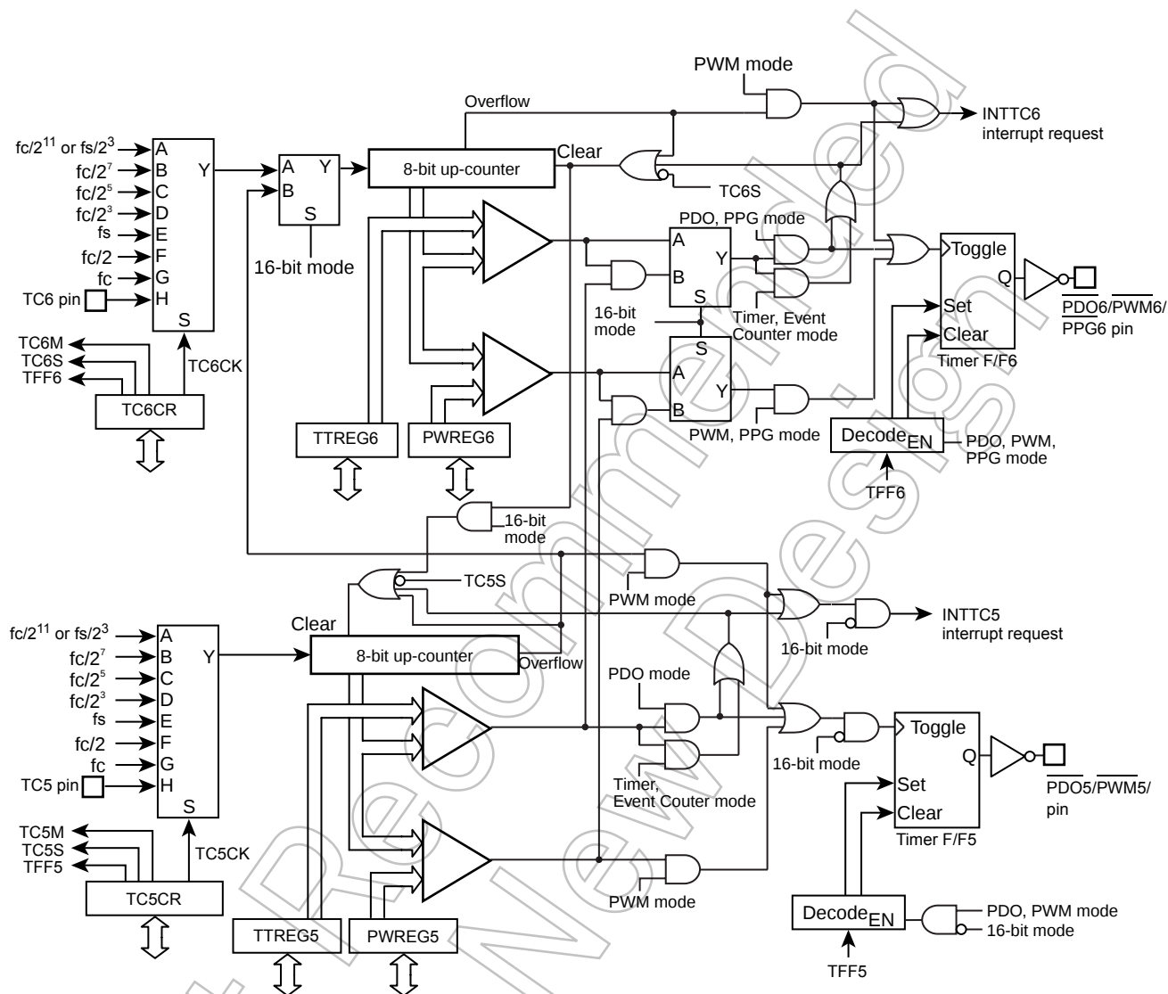
Figure 11-1 8-Bit TimerCounter 5, 6
