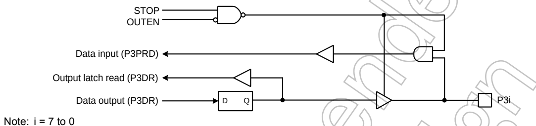
Figure 5-5 Port 3
