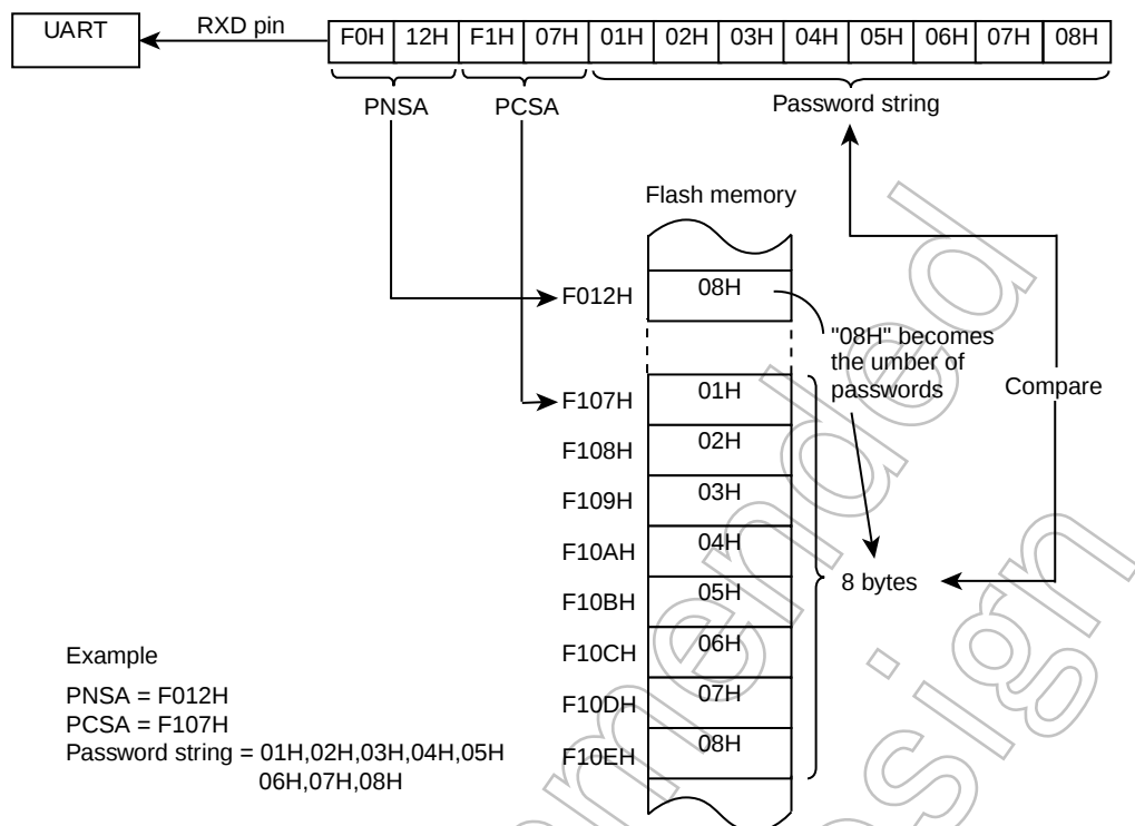
Figure 20-5 Password Comparison
