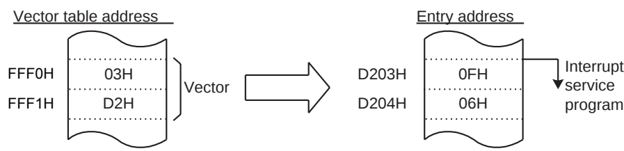
Figure 3-2 Vector table address, Entry address
