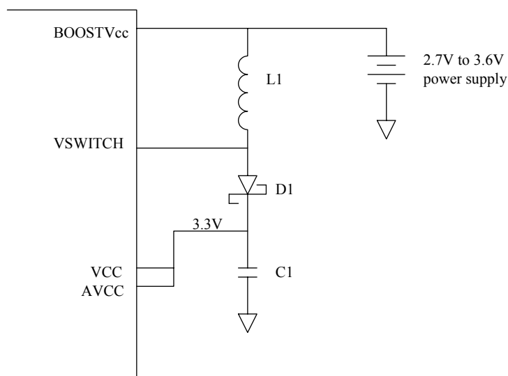
Figure 4-2. Power Supply Connection With Booster
