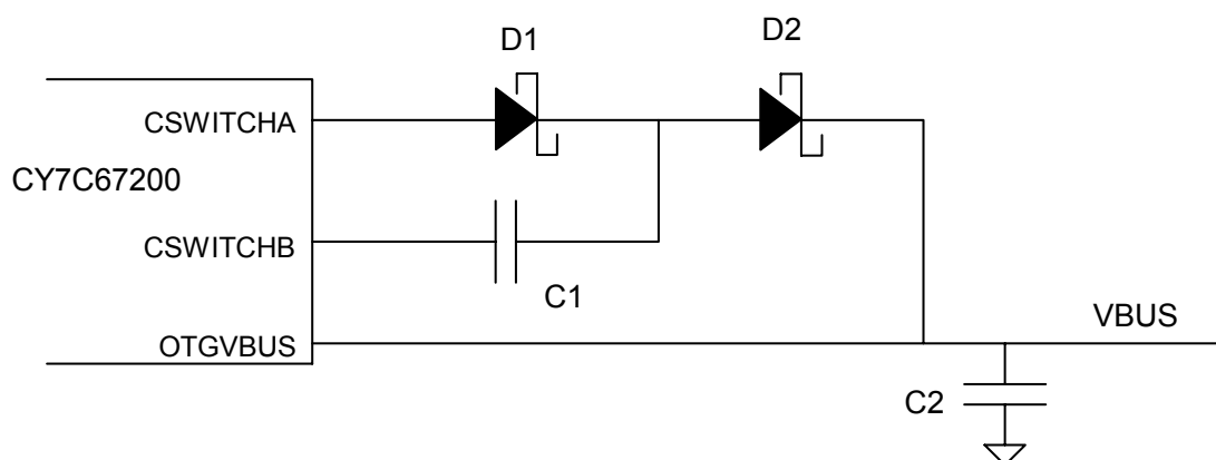
Figure 4-1. Charge Pump
