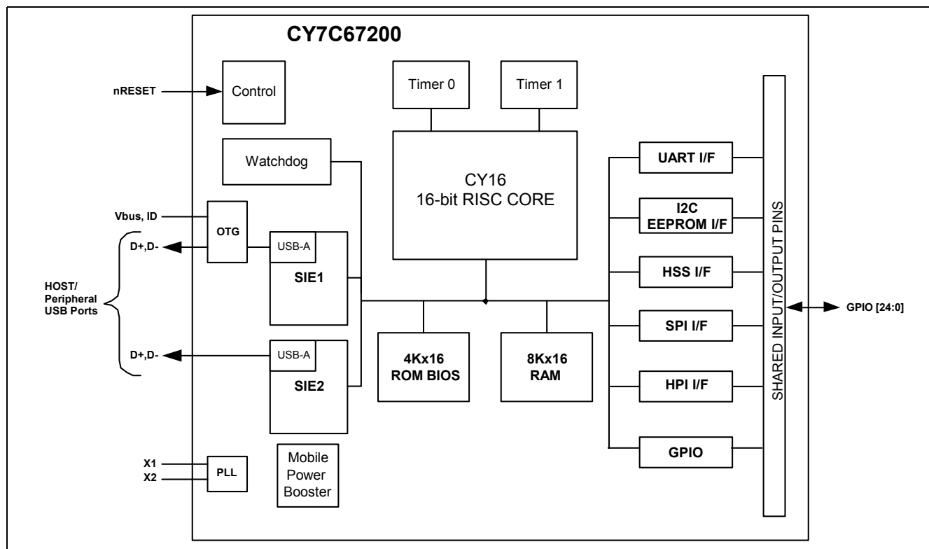
Figure 1-1. Block Diagram
