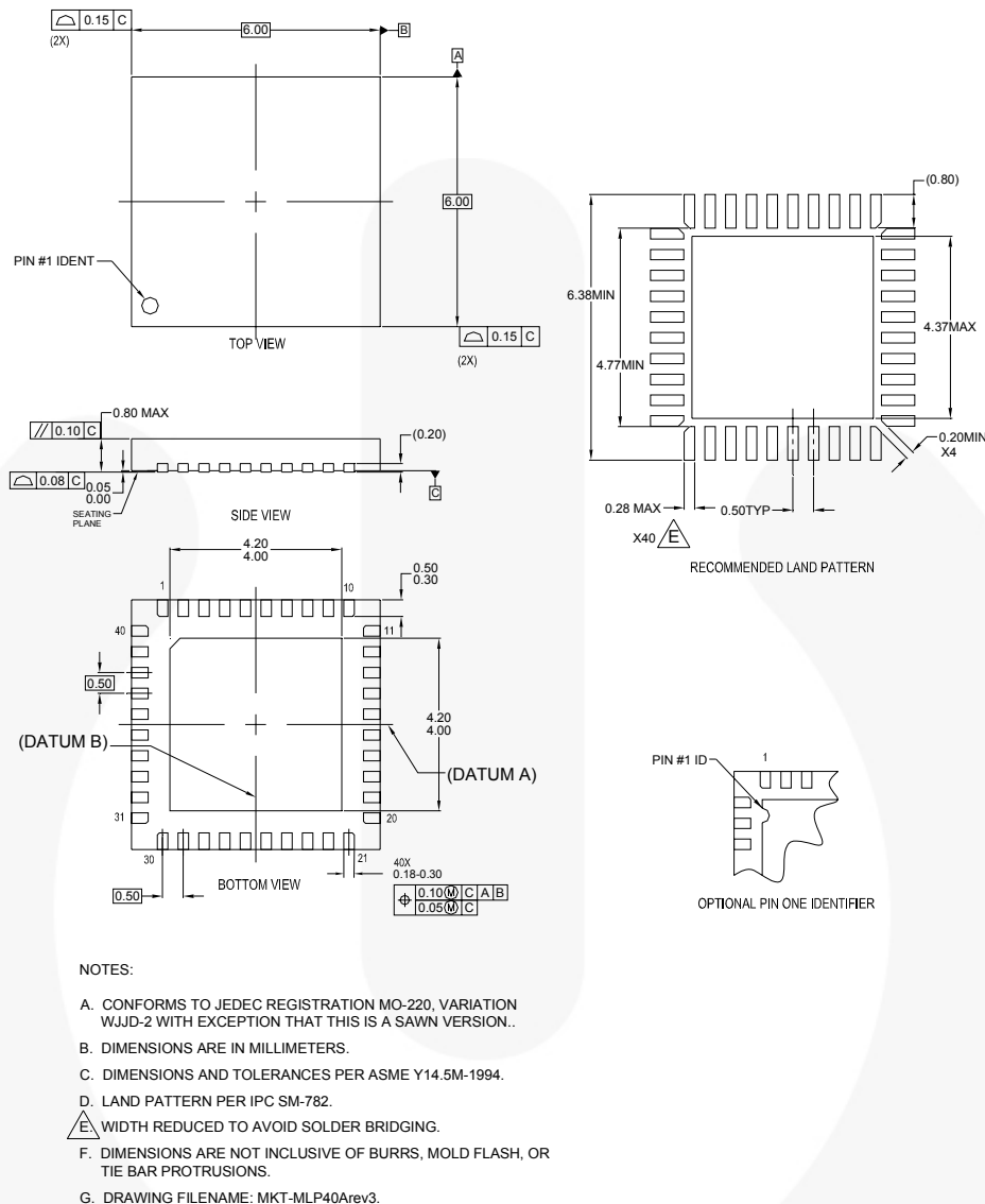
Figure 6. 40-Lead, Molded Leadless Package (MLP), Quad, JEDEC MO-220, 6mm Square
