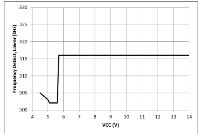
Figure 18. Lower Frequency Detect vs. V_{CC} ( T_J = 25^{\circ}\text{C} )
