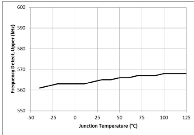
Figure 15. Upper Frequency Detect vs. Temperature (RRAMP = 130 kΩ)
