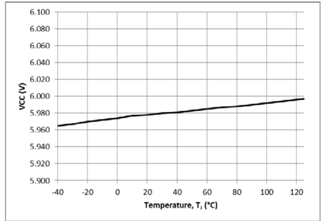
Figure 12. V CC Regulation vs. Temperature (V IN = 10 V)
