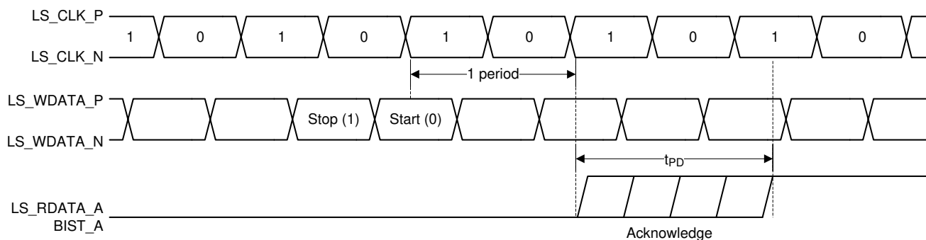
Figure 6-2. Switching Characteristics
