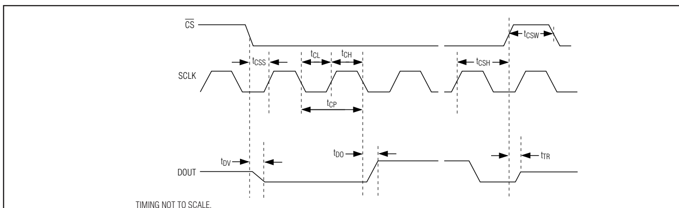
Figure 3. Detailed Serial Interface Timing
