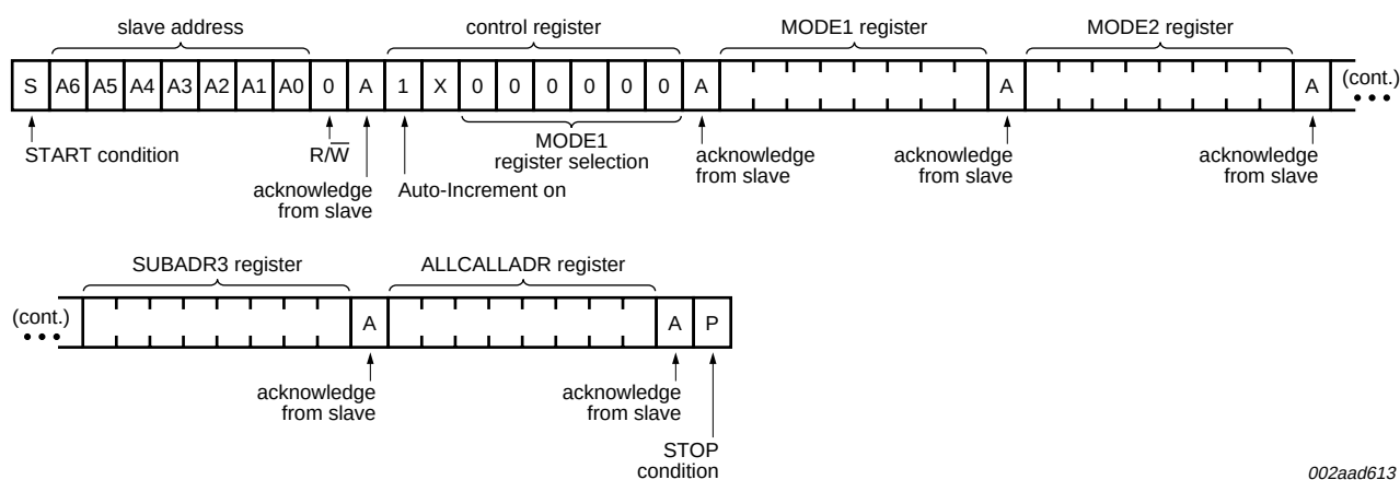
Fig 13. Write to all registers using the Auto-Increment feature
