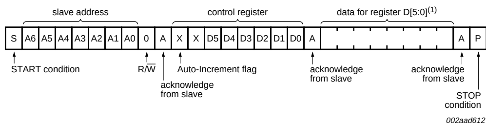
Fig 12. Write to a specific register
