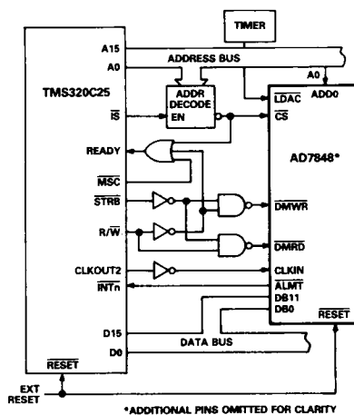
Figure 17. AD7848 – TMS320C25 Interface
