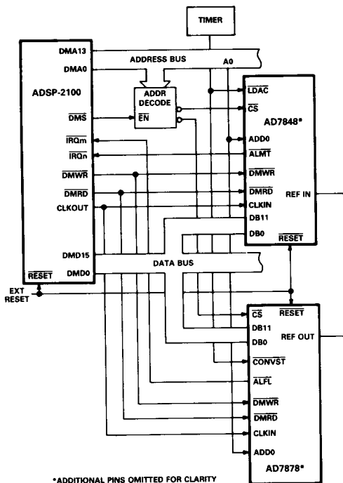
Figure 16. AD7848/AD7878 – ADSP-2100 Interface
