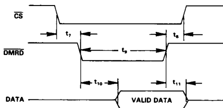
Figure 10. AD7848 Read Operation
