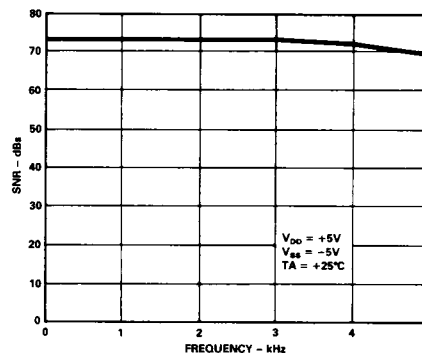
Figure 14. Performance vs. Frequency (No Sample-and-Hold)
