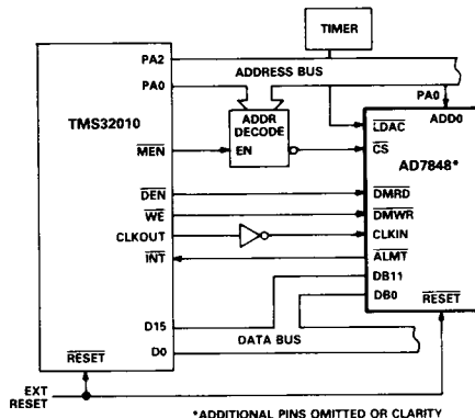
Figure 18. AD7848 – TMS32010 Interface
