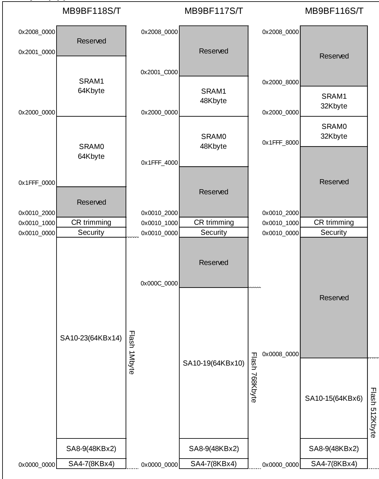
Memory Map (2)
