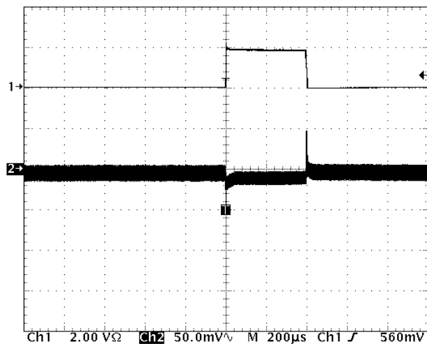
Channel 1: Current sourced into of VDDQ, 2.0 A/div Channel 2: VDDQ output voltage, AC-coupled, 50 mV/div Time base: 200 \mu s/div
