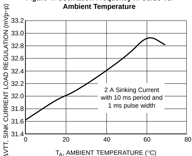
Figure 6. VTT Sink Current Load Regulation vs. Ambient Temperature
