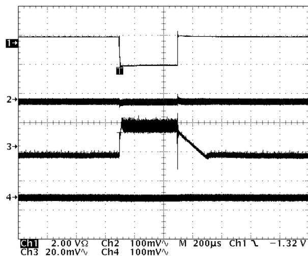
Channel 1: Current sink into of VTT, 2.0 A/div Channel 2: VDDQ output voltage, AC-coupled, 100 mV/div Channel 3: VTT output voltage, AC-coupled, 20 mV/div Channel 4: V1P5 output voltage, AC-coupled, 100 mV/div Time base: 200 \mu s/div
