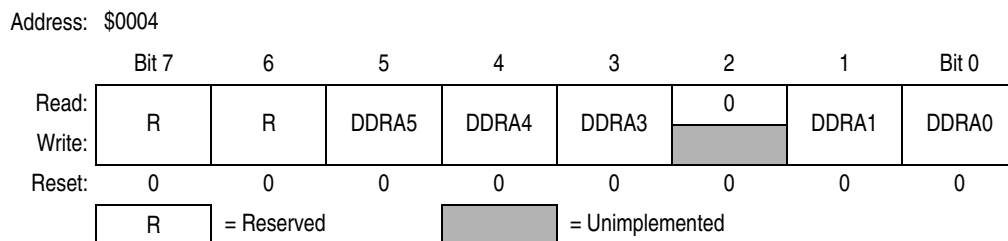
Figure 13-3. Data Direction Register A (DDRA)
