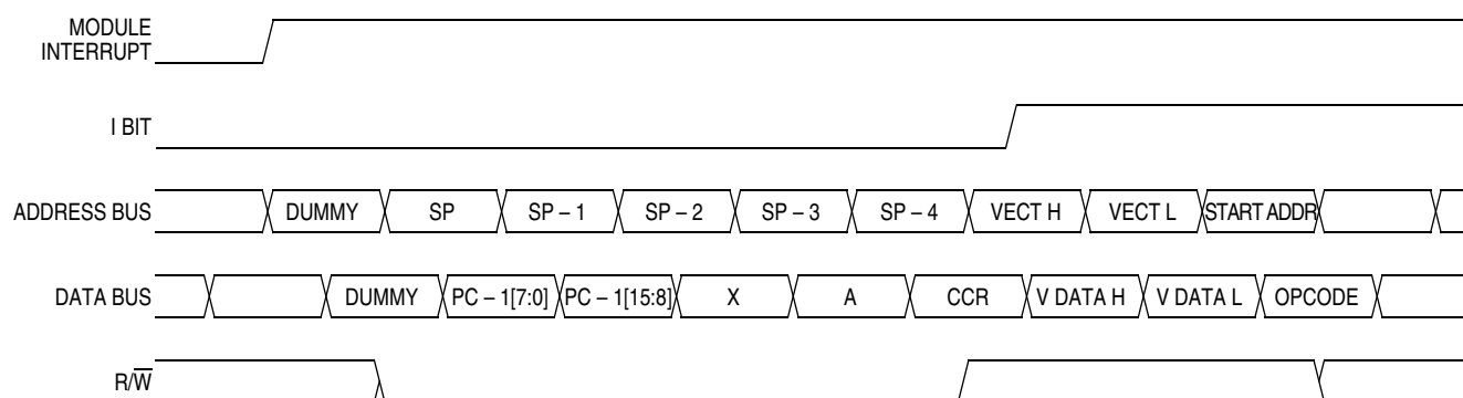
Figure 14-9. Interrupt Entry
