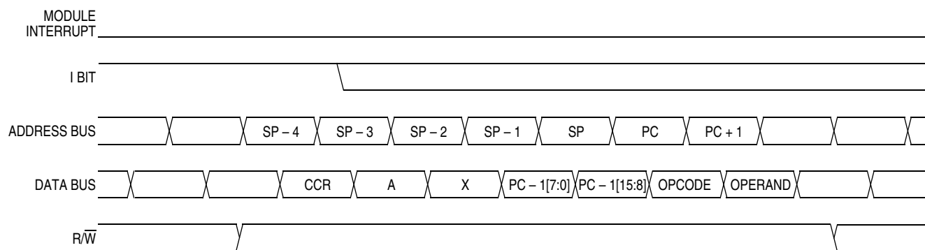
Figure 14-10. Interrupt Recovery
