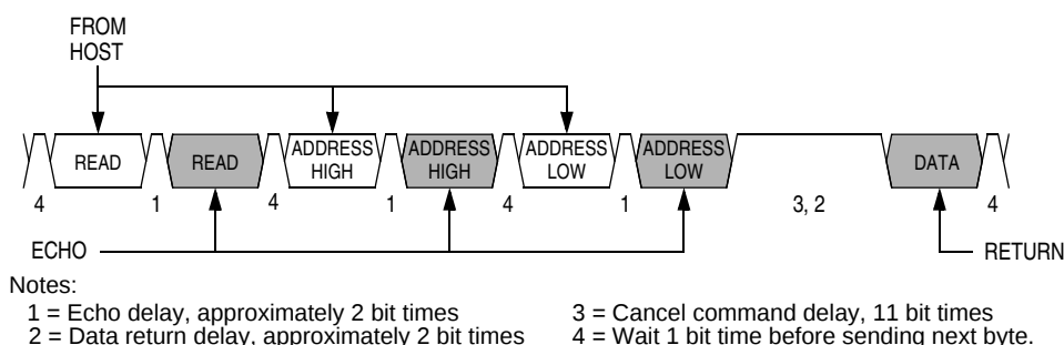
Figure 16-16. Read Transaction
