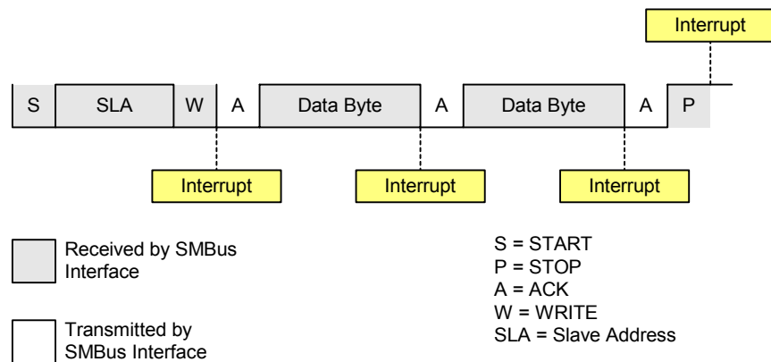
Figure 15.10. Typical Slave Receiver Sequence
