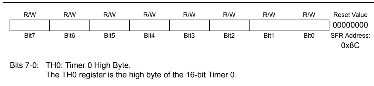
Figure 18.9. TH0: Timer 0 High Byte
