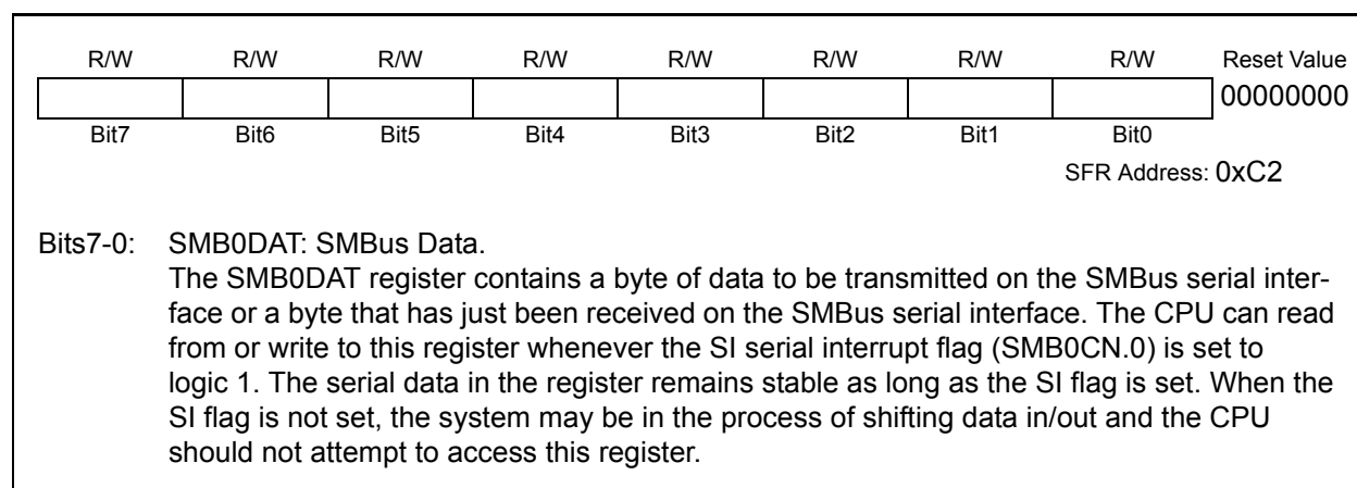
Figure 15.7. SMB0DAT: SMBus Data Register
