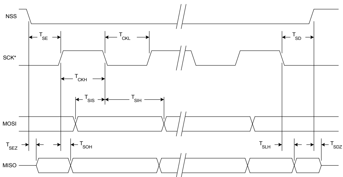
Figure 17.15. SPI Slave Timing (CKPHA = 1)
