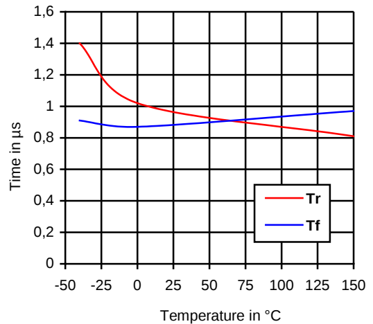
Figure 12: Rise and fall time vs. temperature
