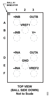
Figure 3. Pin Configuration
