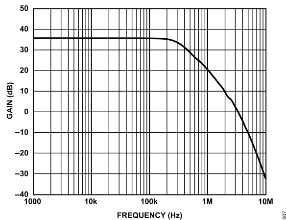
Figure 7. Typical Small Signal Bandwidth ( V_{\text{OUT}} = 200 \text{ mV p-p} )
