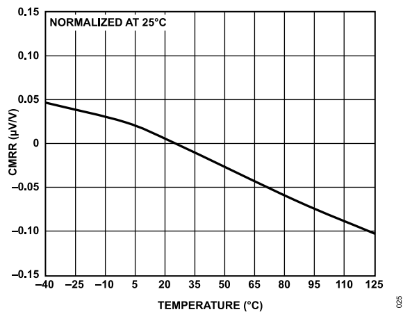
Figure 25. CMRR vs. Temperature
