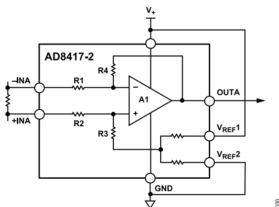
Figure 30. Split Supply
