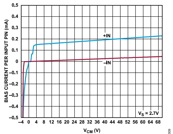
Figure 9. Bias Current per Input Pin vs. V_{\text{CM}}
