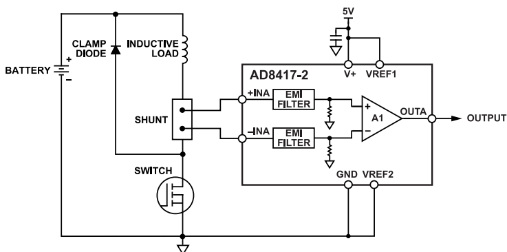
Figure 34. Low-Side Switch
