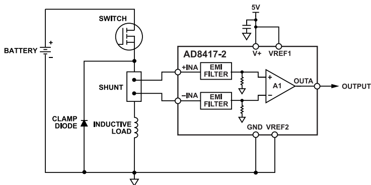
Figure 35. High-Side Switch
