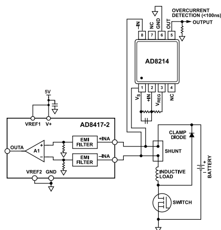
Figure 36. High Rail Current Sensing
