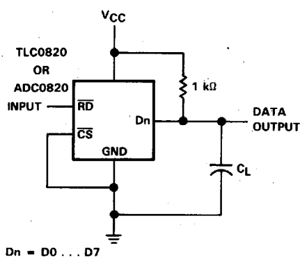
TEST CIRCUIT
