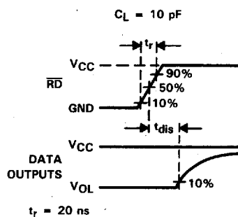
VOLTAGE WAVEFORMS
