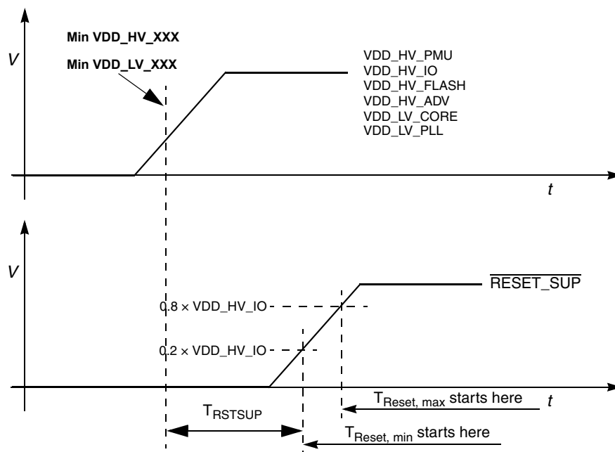
Figure 18. External VREG mode, \overline{\text{RESET\_SUP}} rises after \text{V}_{\text{DD\_HV\_xxx}} are stable
