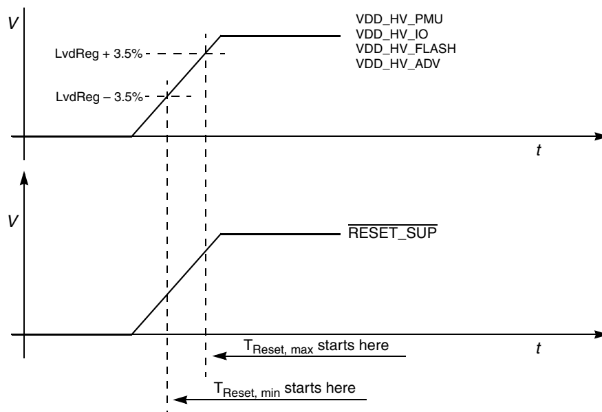
Figure 19. External VREG mode, \overline{\text{RESET\_SUP}} rises with \text{V}_{\text{DD\_HV\_xxx}}
