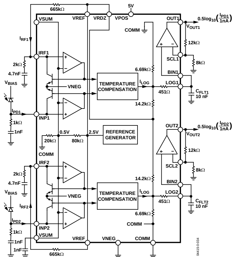
Figure 34. Basic Connections for Fixed Intercept Use
