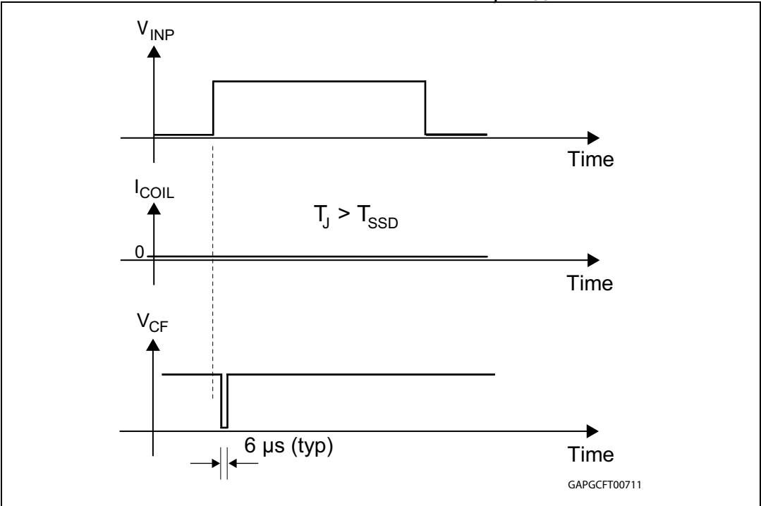
Figure 11. Switch on attempt at T_i > T_{SSD}
