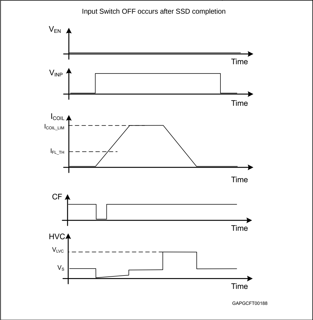
Figure 8. Current limit followed by TSD activation ( T_i = TSD ) (case 1)
