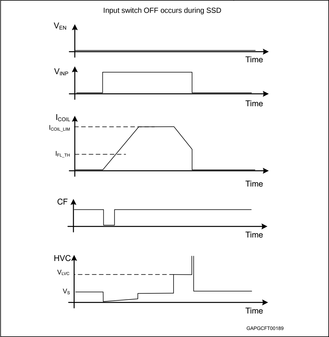
Figure 9. Current limit followed by TSD activation ( T_i = \text{TSD} ) (case 2)
