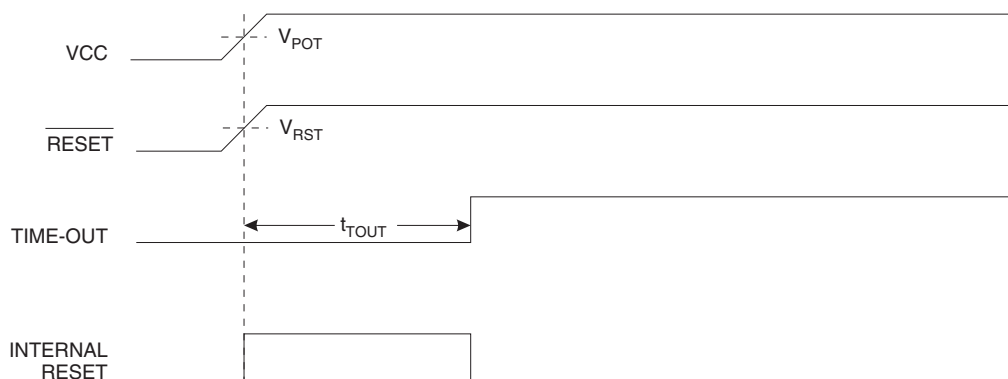
Figure 26. MCU Start-up, \overline{\text{RESET}} Tied to VCC
