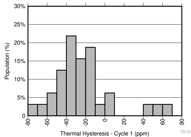
Figure 8-17. Thermal Hysteresis Distribution (Cycle 1) - DBV Package
