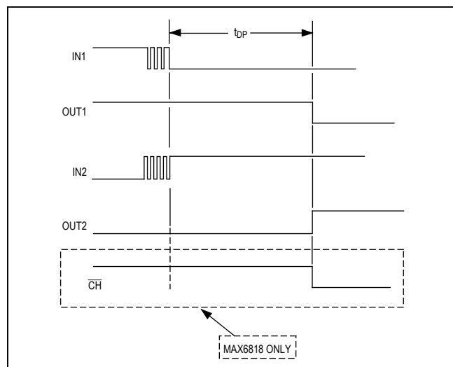
Figure 2. Input Characteristics
