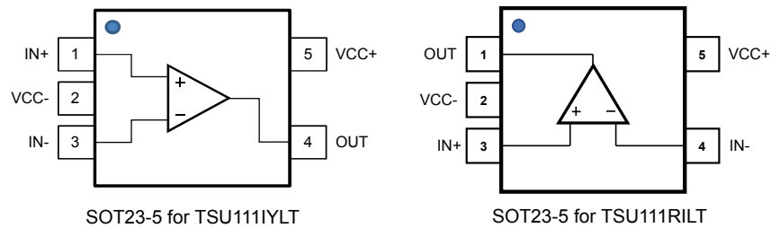
Figure 1. Pin connections for SOT23-5 package (top view)
