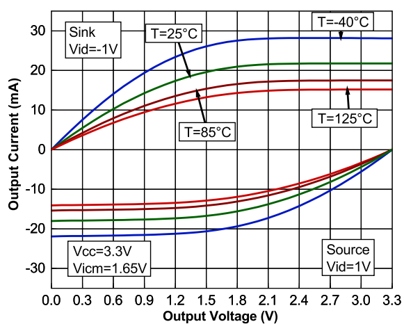
Figure 17. Output characteristics at 3.3 V supply voltage
