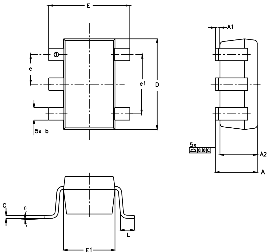
Figure 43. SOT23-5L package outline
