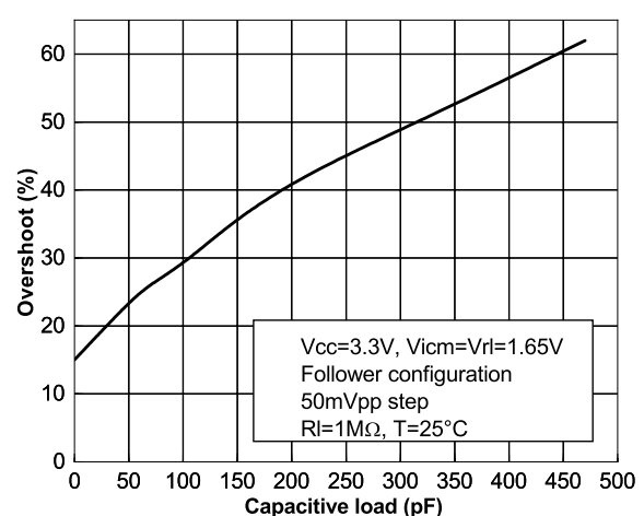
Figure 30. Overshoot vs. capacitive load at 3.3 V supply voltage
