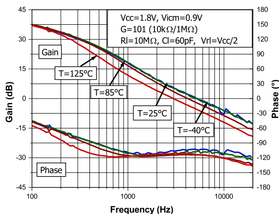
Figure 33. Bode diagram at 1.8 V supply voltage
