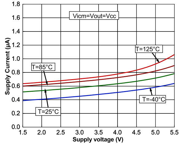
Figure 4. Supply current vs. supply voltage at high V_{ICM}
