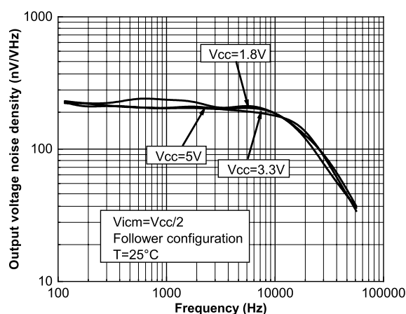
Figure 40. Noise vs. frequency for different power supply voltages
