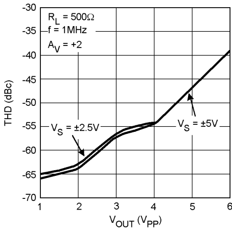
THD vs. Output Swing
