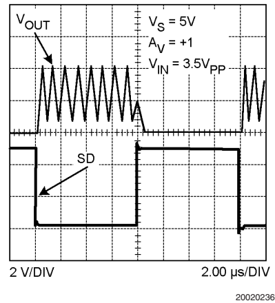
FIGURE 4. Output Held Low by Active Pull-Down Circuit
