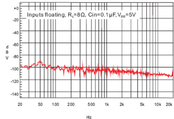
12. Noise Floor
