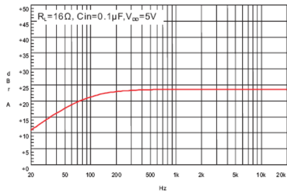
11. Frequency Response
